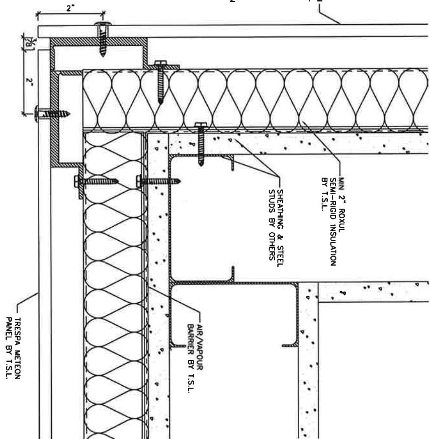
2 OUTSIDE CORNER PLAN SCALE: 6"=1'-0" REF: NONE
